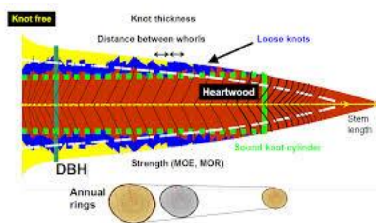
Figure 14 Picture virtual Stem (Stem profile) source Biometria, SLU
