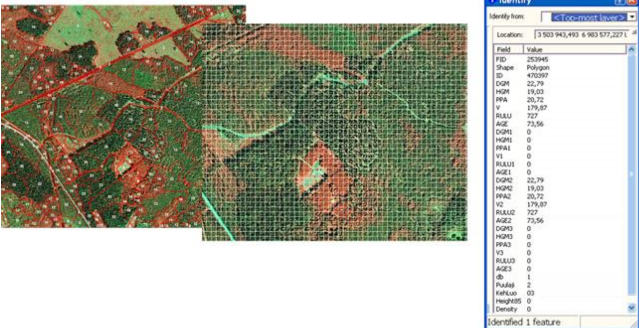
Figure 9 Forest inventory primary unit (Paananen 2019)
