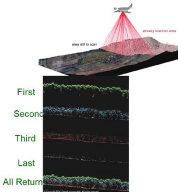
Figure 7 Airborne laser scanning method (Paananen 2019)
